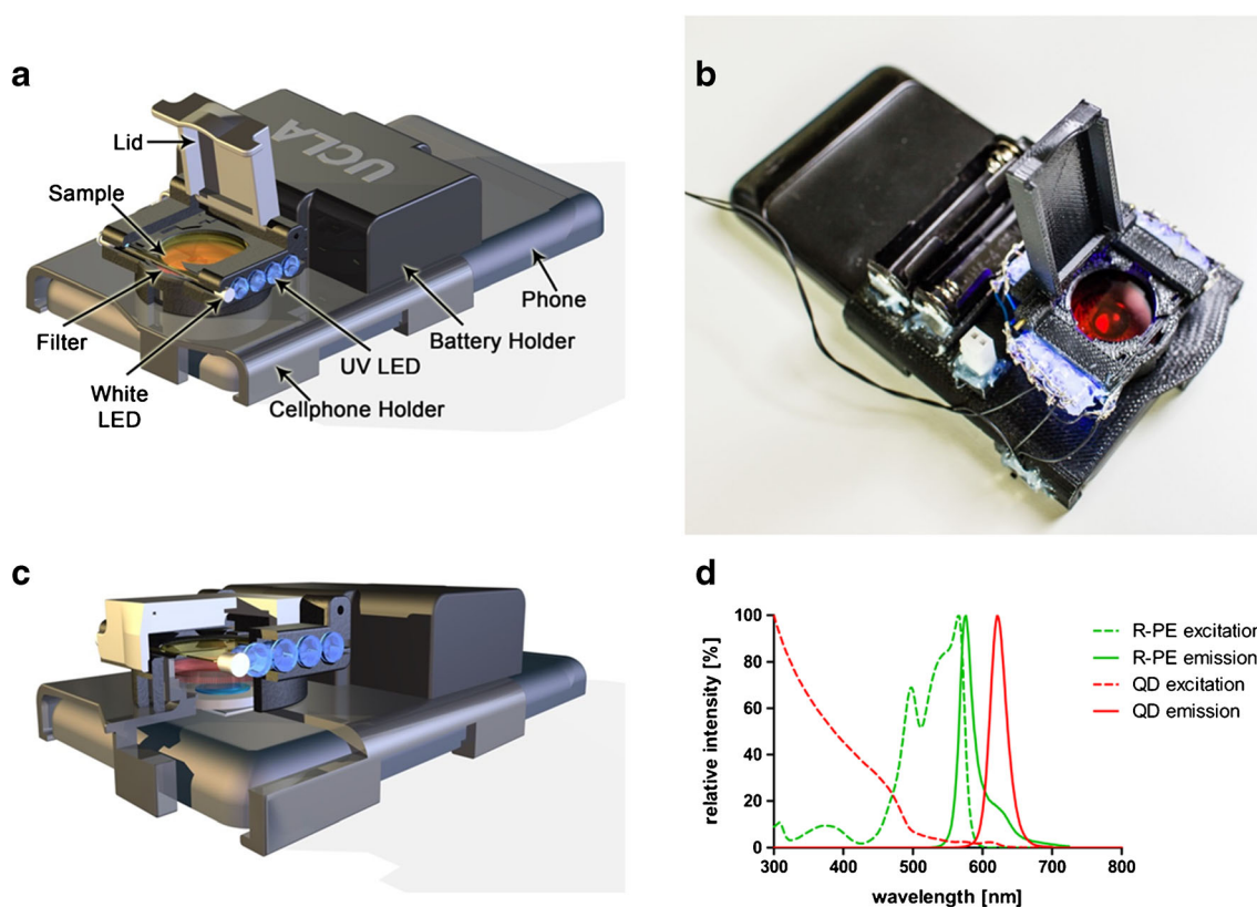
Fig. 1 Schematic overview (a, c) and a picture (b) of the cellphone attachment for the detection of rbST biomarker in milk extracts. Excitation (dotted lines) and emission (solid lines) spectra (d) of R-phycoerythrin (R-PE, green) and 625-nm emitting quantum dots (QD, red)
